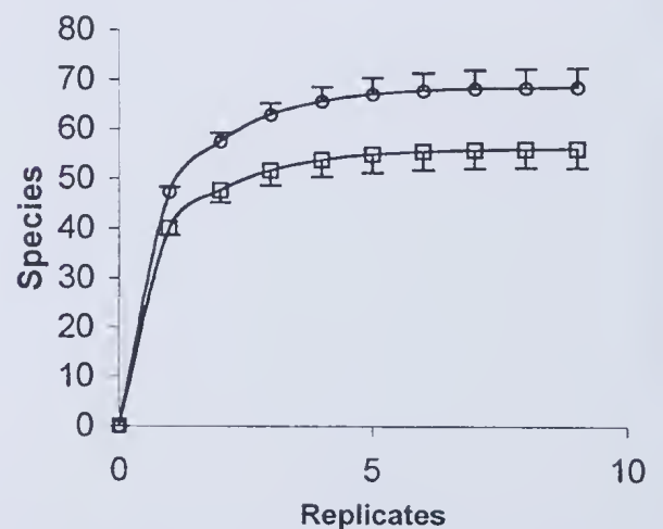
Figure 6. Accumulation of invertebrate species at Toolibin ( \square ) and Walbyring (o) Lakes with increasing numbers of replicates (see text for details); error bars are \pm 1 SE.
